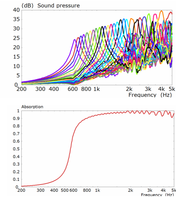
Figure 5 Top: pressure response at closed end of each separate absorber channel. Bottom: absorption spectrum of whole absorber.
