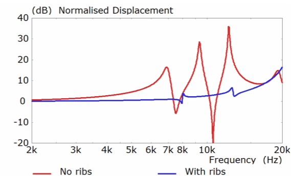
Figure 13 Simulated displacement of tangerine waveguide
