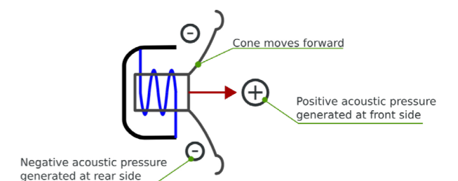
Figure 2 - Generic driver
