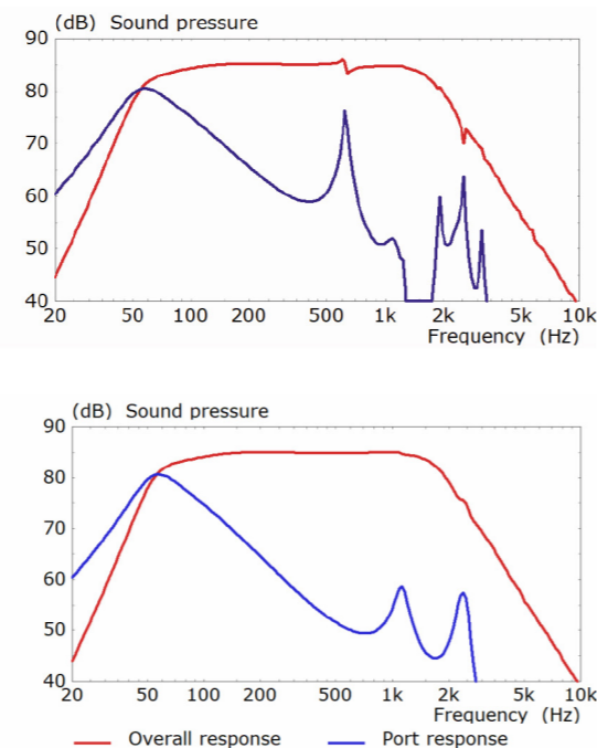
Figure 29 Simulated comparison of the port and total speaker outputs with unoptimised (top) and optimised (bottom) port location.
