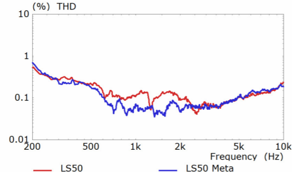
Figure 23 THD, measured as a percentage of the fundamental level 90dB SPL at 1m for LS50 (red) and LS50 Meta (blue).
