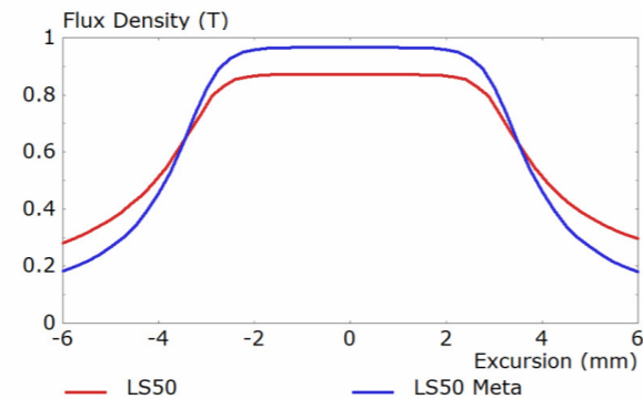
Figure 21 Comparison of flux density in the gap.
