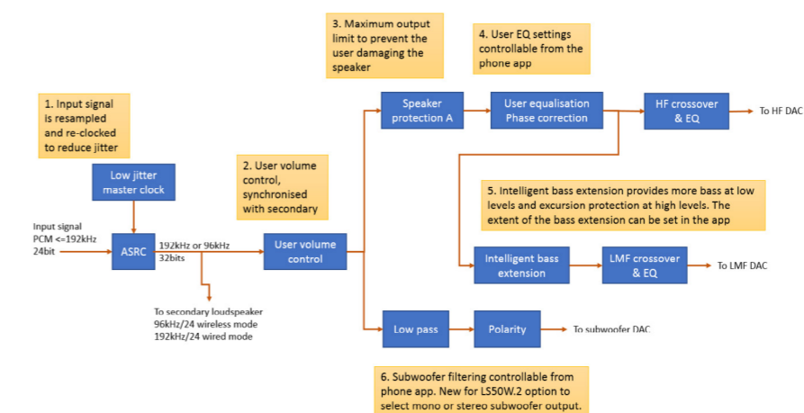
Figure 46 - DSP Details
