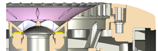
Figure 39 Cross section of complete Uni-Q driver and trim ring
