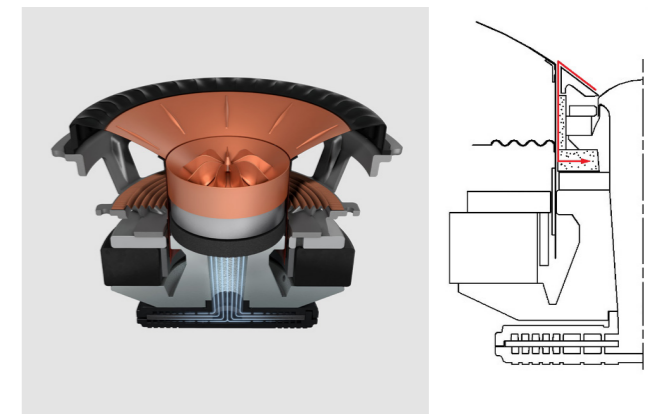
Figure 14 Uni-Q driver with damped, optimised gap
