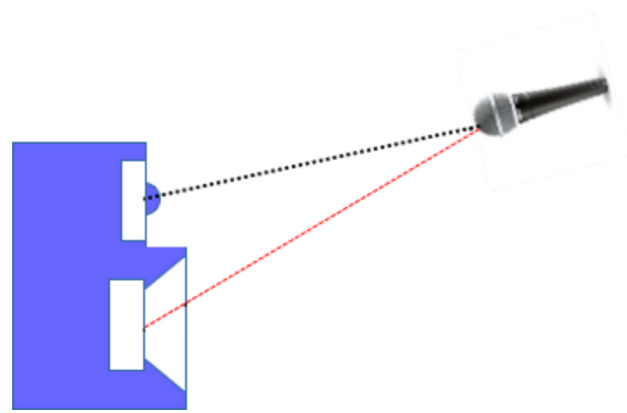
Figure 52 Conventional speaker, mic. above axis.
