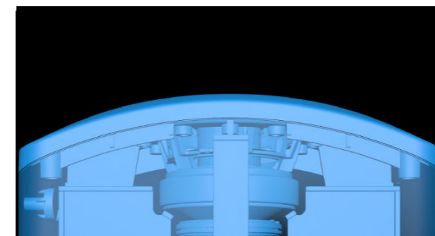
Figure 27 Low-diffraction Baffle
