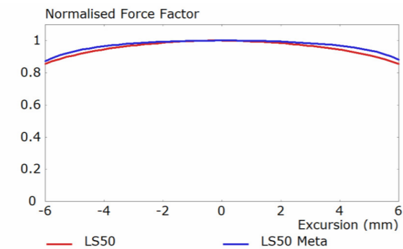
Figure 22 Comparison of bass/midrange force factor
