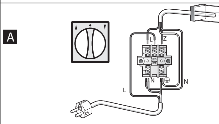
Mounting instruction
